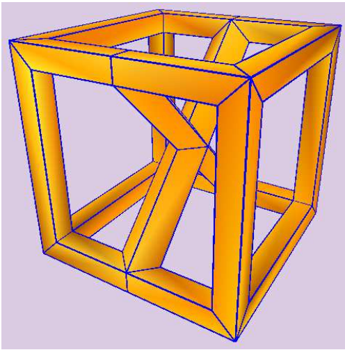
(c) Given Mesh
