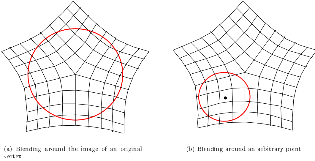
Figure 3: Parameter space for a vertex of degree 5 and for an arbitrarily selected point.
