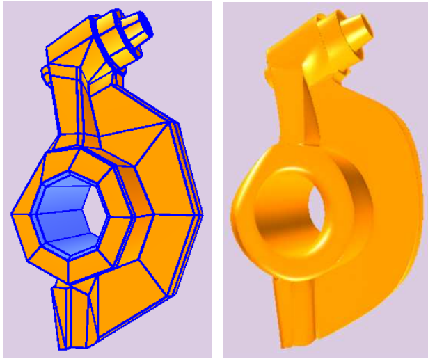
(a) Given Mesh
